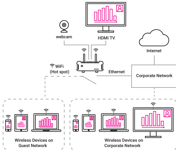
HHO+ Direct mode
